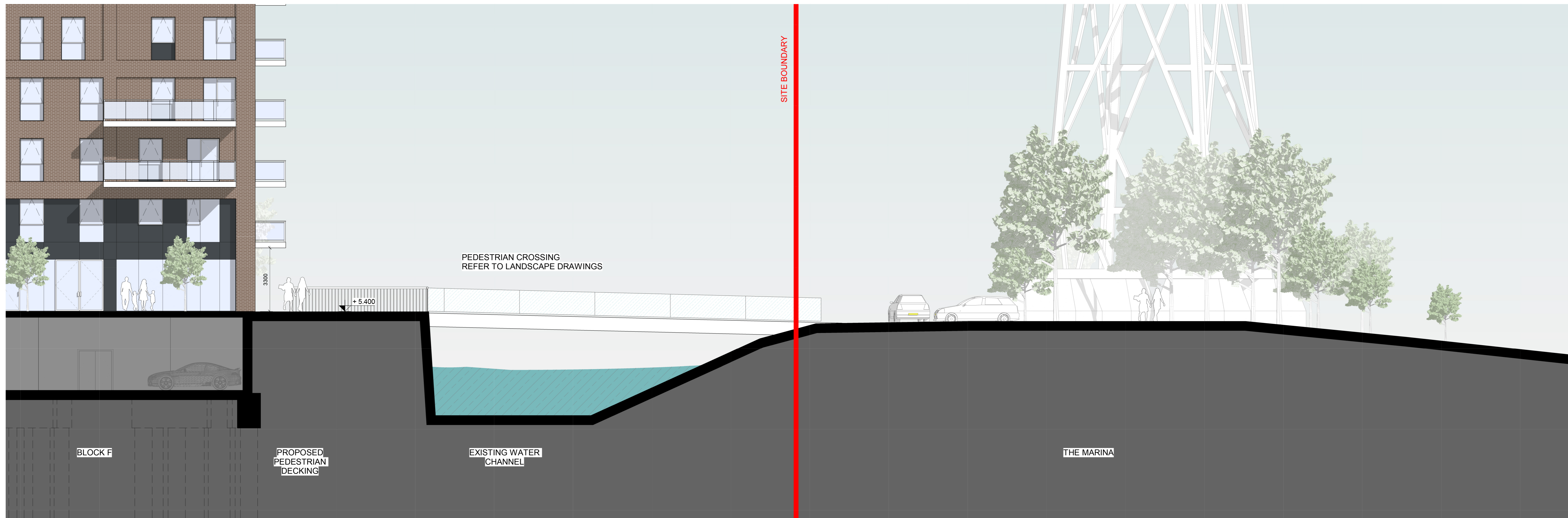
2 CONTEXTUAL SITE SECTION F-F - DETAIL 1:100
